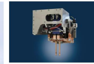
Robot welding guns for single-sided resistance spot welding
